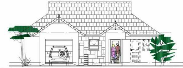
SOUTH ELEVATION
